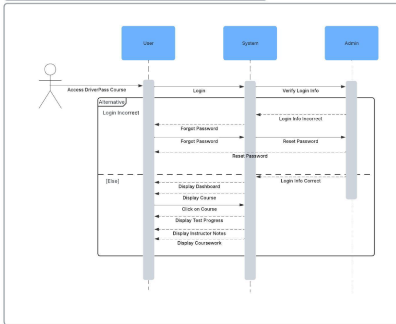
DriverPass UML Sequence Diagram
