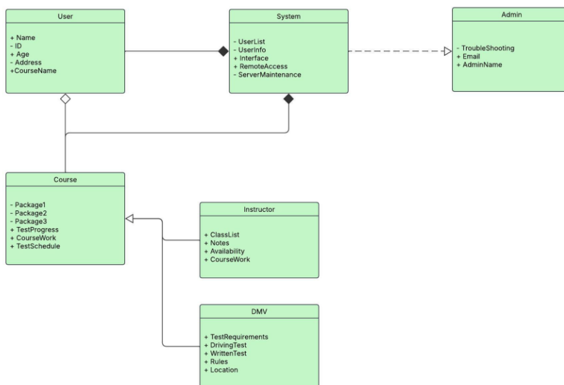
DriverPass UML Class Diagram
